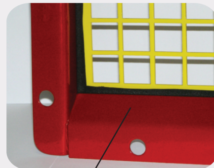
45 degree flange on interior of door prevents fines from accumulating.
