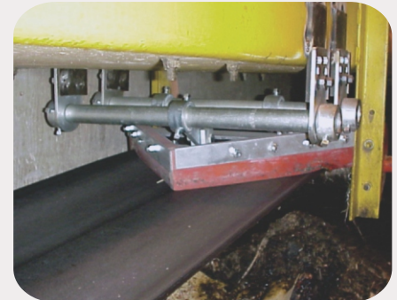
Heavy Duty V-Plow shown installed.
