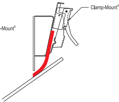
Dura-Tuff™ Urethane Skirting
