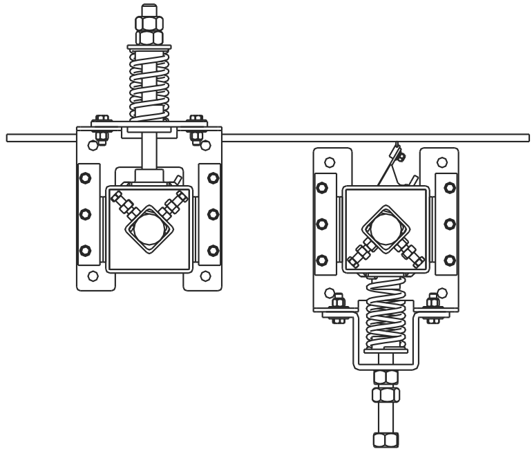
Figure 1. Typical Cleaner Mounting Locations
