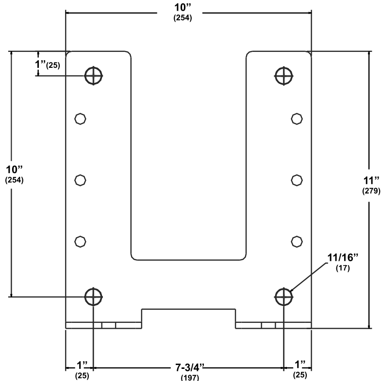
Figure 2. Mounting Bracket Dimensions
