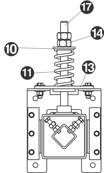
PULL-UP Position
