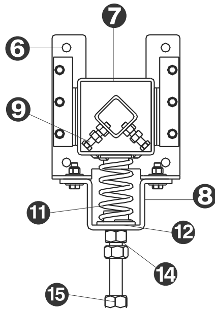
PUSH-UP Position
