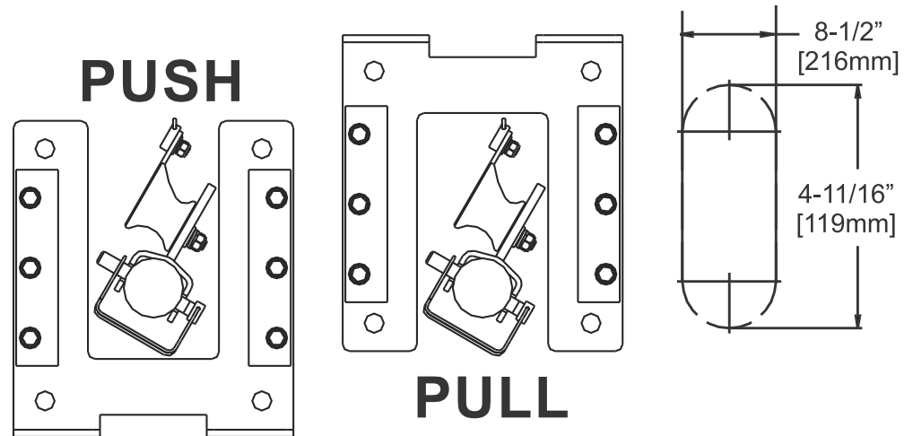
Figure 4. Chute Openings Dimensions
