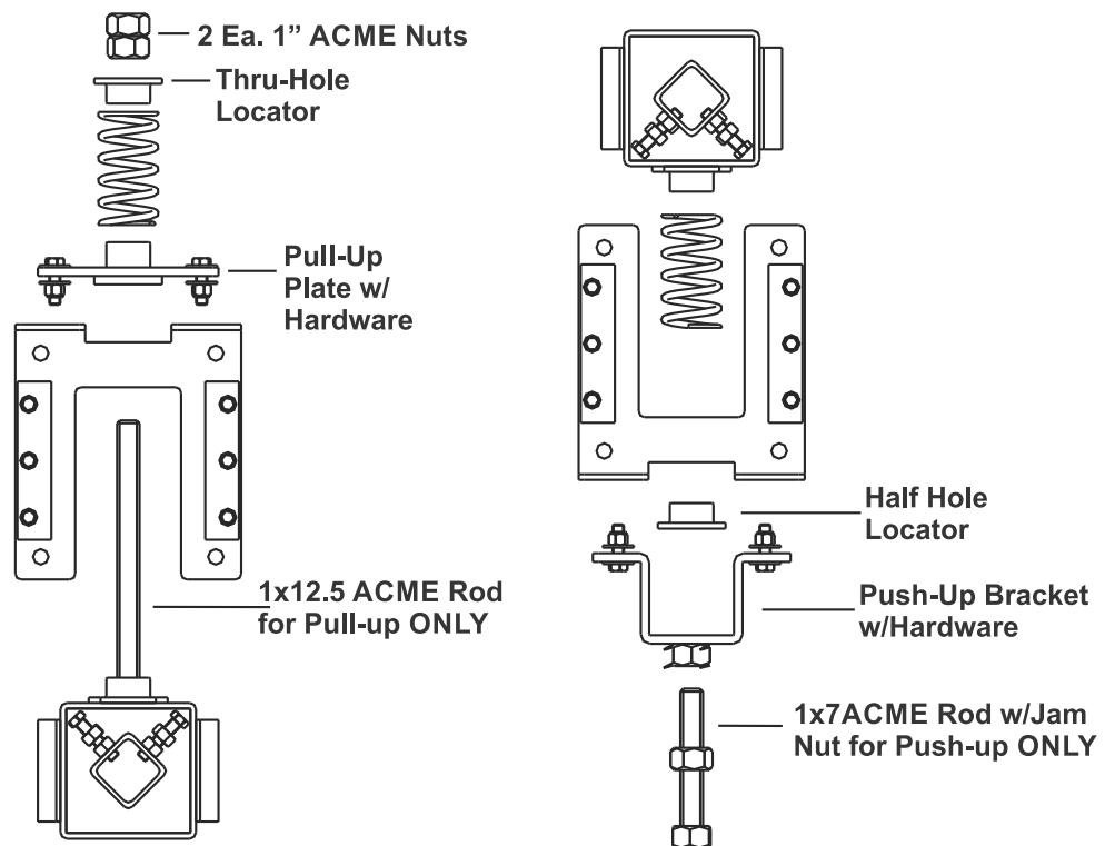
Figure 5. Duo-Spring Tensioner Assembly: Pull-Up (left) and Push-Up (right) Tensioners
