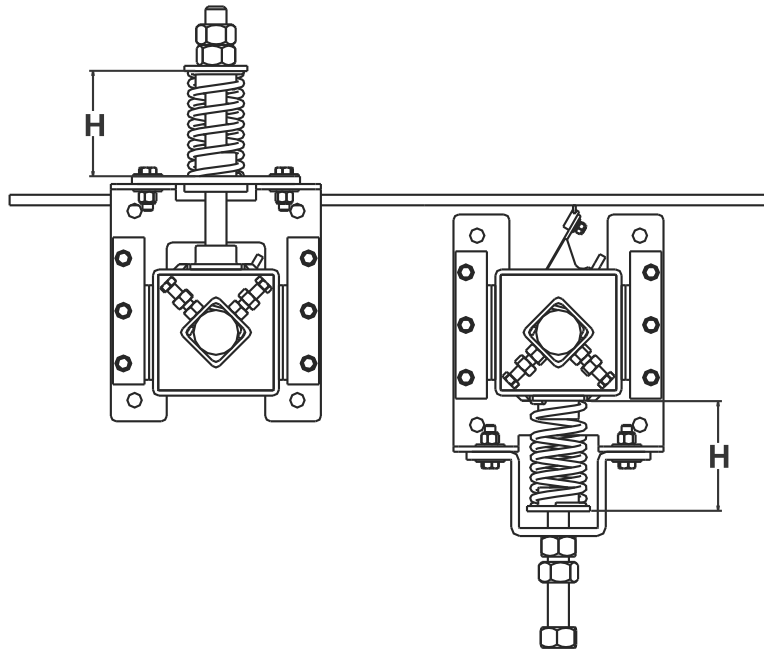
Spring Height (H) Measurement Location
