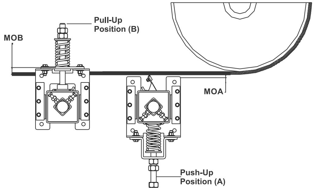
Figure 3: Mounting Bracket Height Locations for Pull-Up & Push-Up Positions
