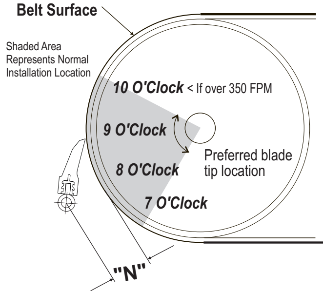
Figure 1: Typical Mounting Position *Note: \pm 1/4" tolerance
