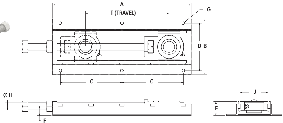
WIDE SLOT TAKE-UP FRAME (WSTU)
