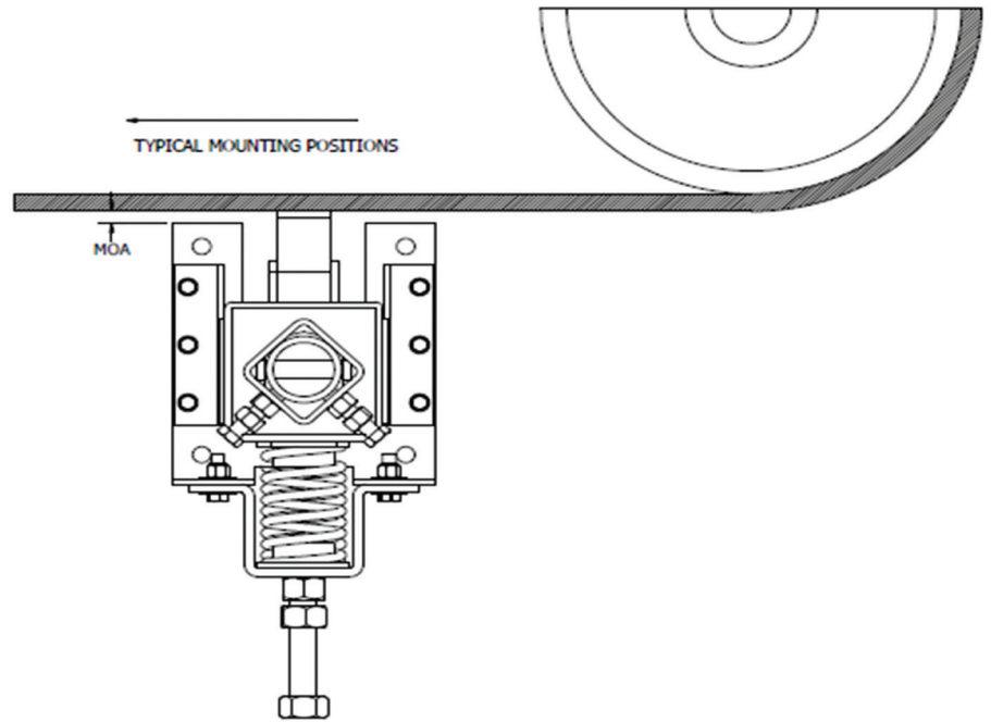
Figure 3. Typical Cleaner Mounting Locations
